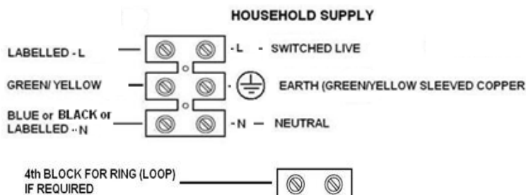
Details of terminal wiring at (5)
